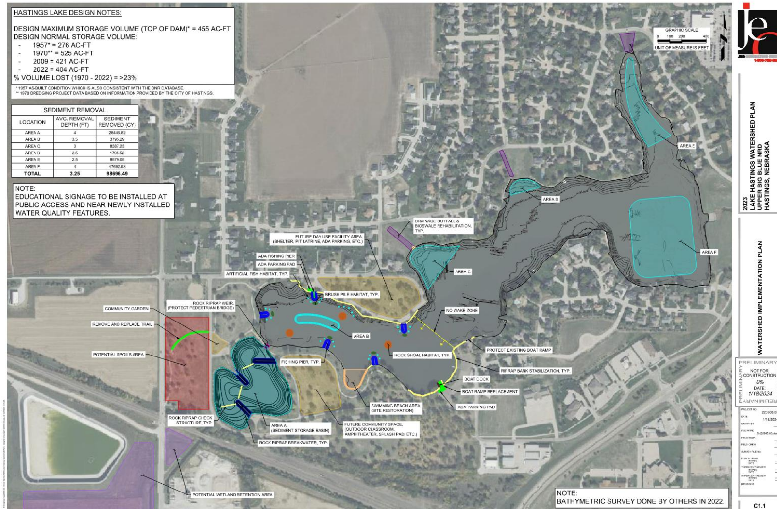
Figure 12: Conceptual Drawing of Proposed In-Lake BMPs
